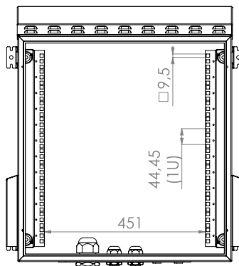
INSIDE VIEW
